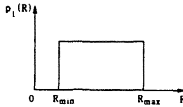
Fig. 4. The distribution function p_1(R) .
